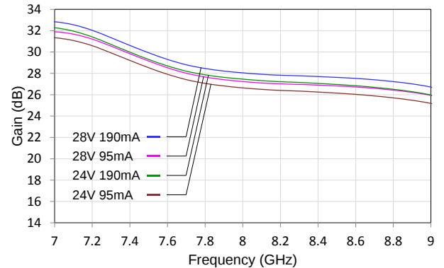
Gain vs. Frequency vs. Bias V_{D1} = V_{D2} = 6\text{ V} , I_{D1} + I_{D2} = 1000\text{ mA} , V_{G12} = -0.65\text{ V} Typical
