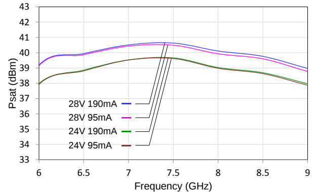
Psat vs. Frequency vs. Bias
