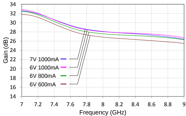
Gain vs. Frequency vs. Bias V_{D3} = 28\text{ V} , I_{D3} = 190\text{ mA} , V_{G3} = -2.6\text{ V} Typical
