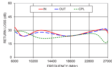
ZCDC10-06263-S+ RETURN LOSS
