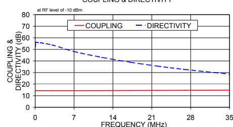
PDC-15-6-75 COUPLING & DIRECTIVITY
