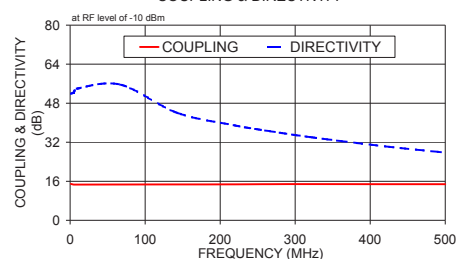
PDC-15-21+ COUPLING & DIRECTIVITY
