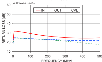
PDC-15-21+ RETURN LOSS
