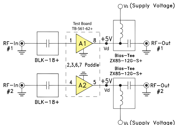
Fig 1a. Block Diagram of Test Circuit used for characterization. (DUT tested in Mini-Circuits Test board TB-561-62+, except for IP2).
