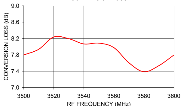
MCA-36FLH+ CONVERSION LOSS
