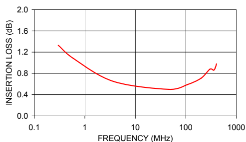
TX1-1 INSERTION LOSS
