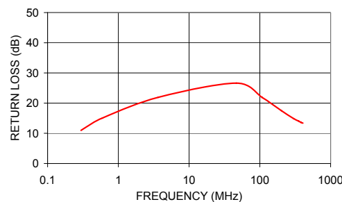
TX1-1 INPUT RETURN LOSS
