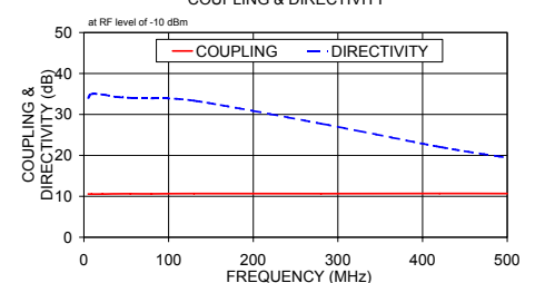
LRDC-10-1J COUPLING & DIRECTIVITY
