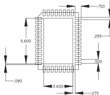
LAND PATTERN
