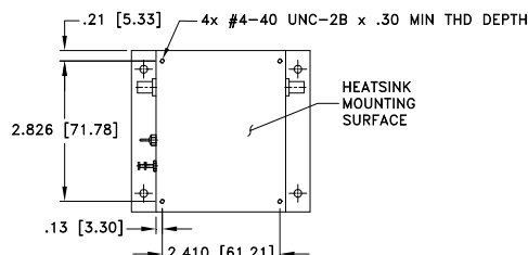
MOUNTING INFORMATION FOR MODELS WITHOUT HEATSINK
