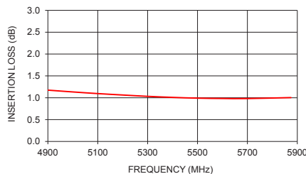
TCW2-63+ INSERTION LOSS
