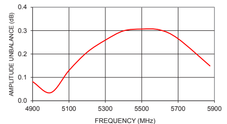
TCW2-63+ AMPLITUDE UNBALANCE
