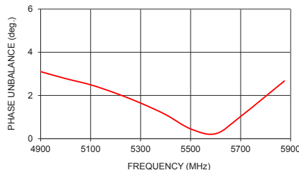
TCW2-63+ PHASE UNBALANCE
