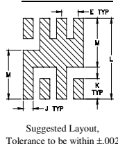
PCB Land Pattern
