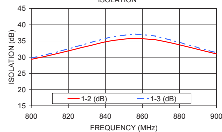
ZN3PD-900 ISOLATION
