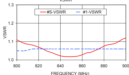
ZN3PD-900 VSWR
