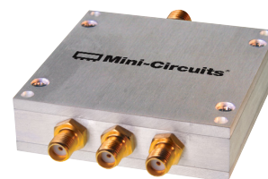
CASE STYLE: UU181 Connectors Model SMA ZN3PD-900W-S
