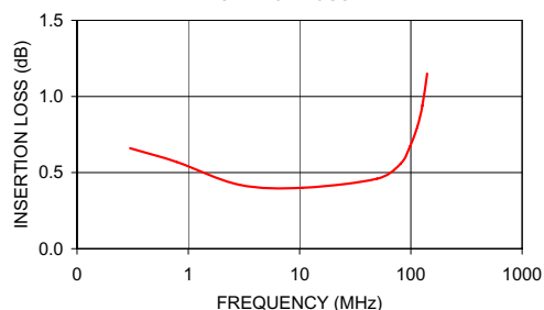
T8-1T-KK81 INSERTION LOSS
