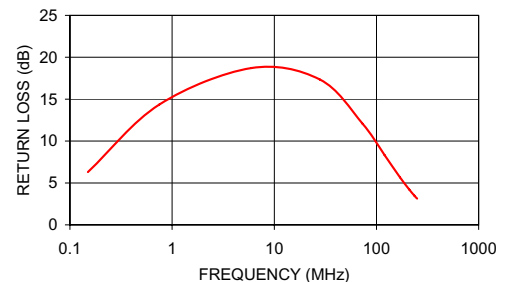
T8-1-X65 INPUT RETURN LOSS
