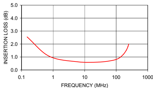
T8-1-X65 INSERTION LOSS
