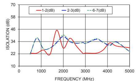
ZN8PD1-53-S+ ISOLATION
