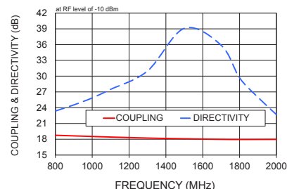
ZNDC-18-2G-S+ COUPLING & DIRECTIVITY
