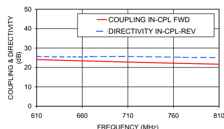
SYBD-22-82HP+ COUPLING & DIRECTIVITY
