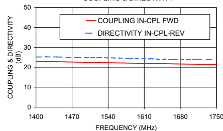
SYBD-22-172HP+ COUPLING & DIRECTIVITY
