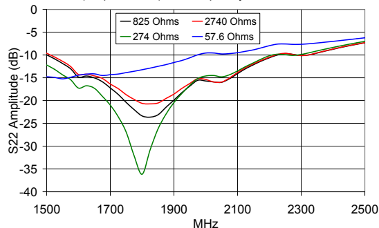
S22 (Amplitude,dB) Vs. Frequency and R1 Values
