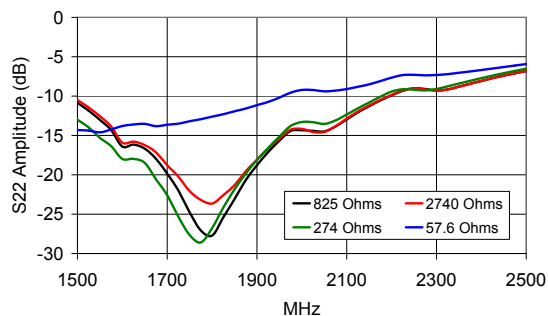
S22 (Amplitude, dB) vs. Frequency and R1 Values
