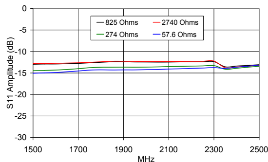
S11 (Amplitude,dB) Vs. Frequency and R1 Values
