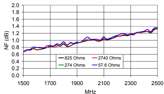
Noise Figure (dB) vs. Frequency and R1 Values
