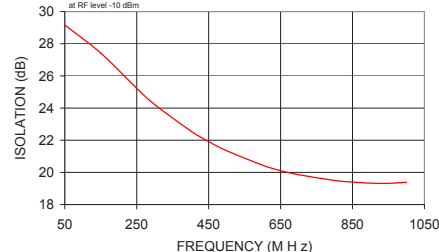
SBTC-2-10-5075 ISOLATION
