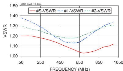
SBTC-2-10-5075 VSWR
