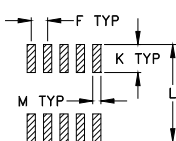
PCB Land Pattern
