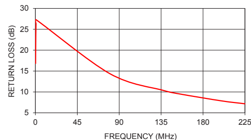
ADT1.5-2+ INPUT RETURN LOSS
