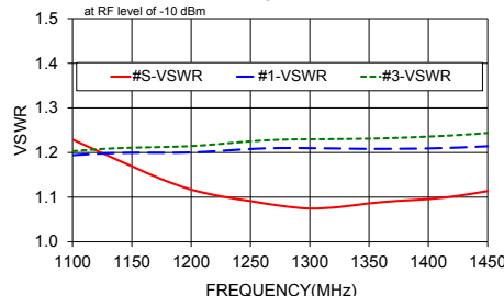
ZX10-4-14-S+ VSWR
