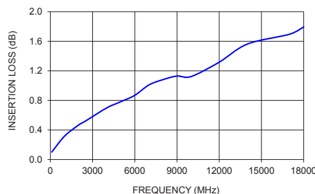
141-32SM+ INSERTION LOSS
