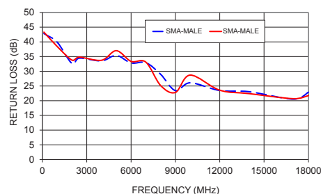
141-32SM+ RETURN LOSS
