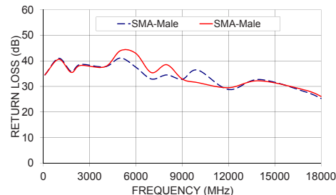
141-22SM+ RETURN LOSS
