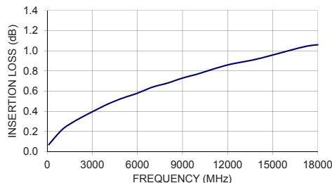
141-22SM+ INSERTION LOSS
