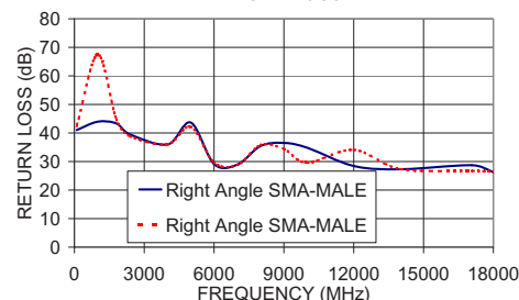
086-9SMR+ RETURN LOSS
