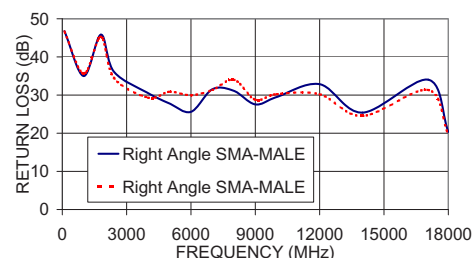
086-7SMR+ RETURN LOSS
