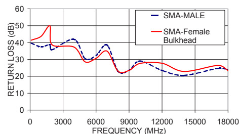
086-6SBSM+ RETURN LOSS
