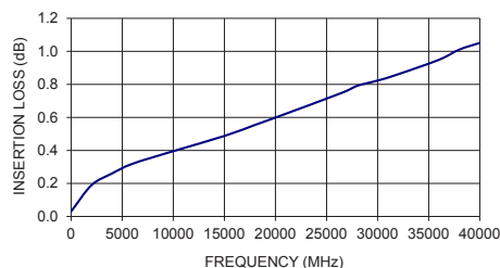
086-6KM+ INSERTION LOSS
