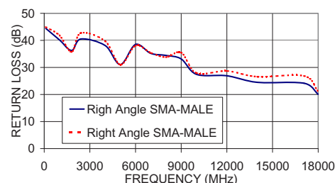
086-2SMR+ RETURN LOSS
