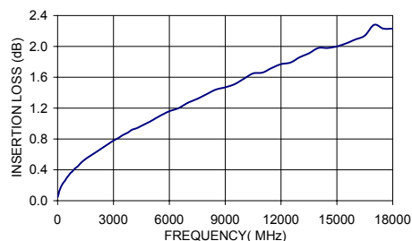
086-24SM+ INSERTION LOSS
