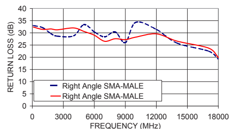
086-18SBSMR+ RETURN LOSS
