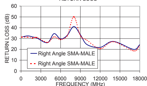
086-10SMR+ RETURN LOSS
