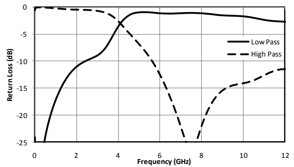
Fig. 3. Return loss.
