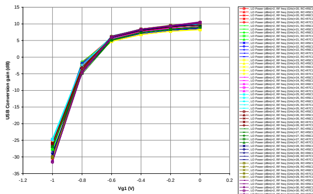
XUI009-BD_5samples: USB Conversion gain (dB) vs. Vg1 (V) IF1_ONLY = 1.84 GHz, -10dBm, LO = 0, 2 & 4 dBm
