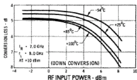
Conversion Loss vs. RF Input Power
