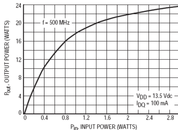
Figure 3. Output Power versus Input Power, 13.5 Vdc
