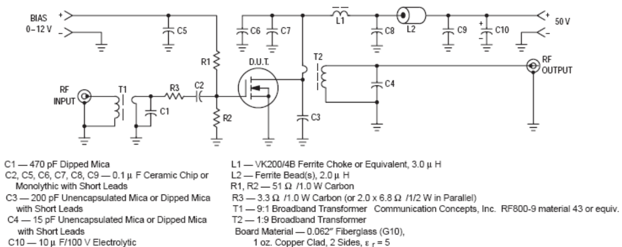
Figure 1. 30 MHz Test Circuit
